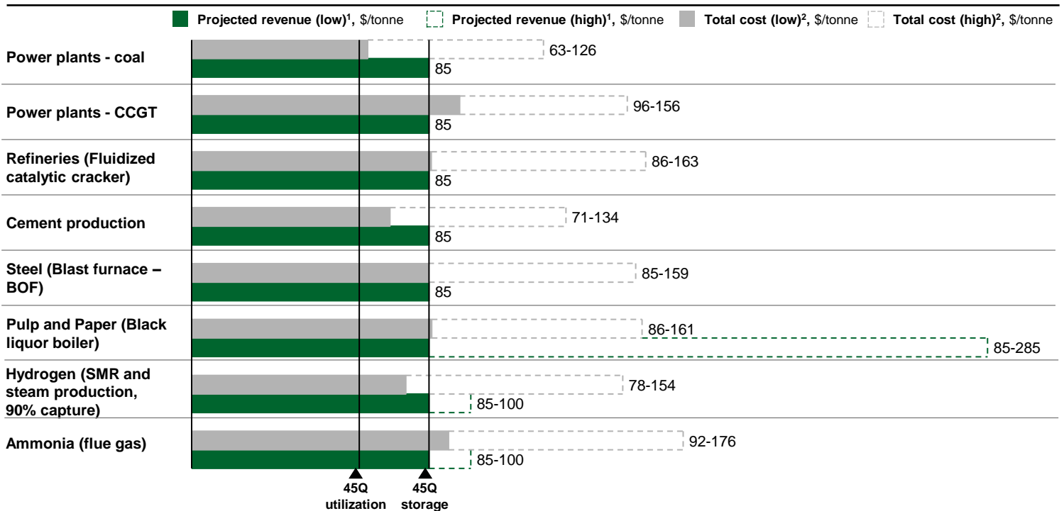
Figure 14: Lower purity point sources require further cost reductions or additional revenue streams
