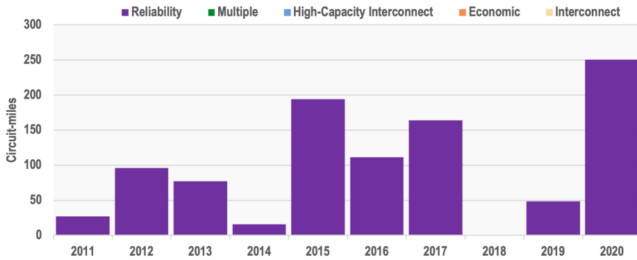
Circuit-miles of new or rebuilt transmission lines ( \geq 100 kV) energized between 2011 and 2020 by project driver.
