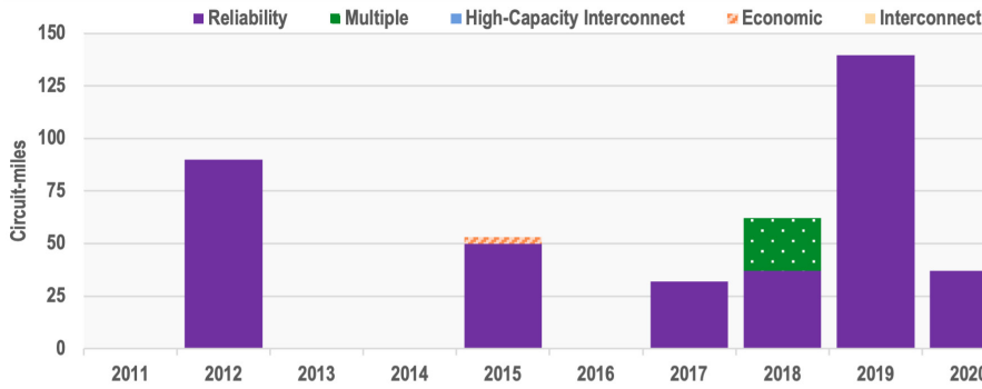
Circuit-miles of new or rebuilt transmission lines (≥ 100 kV) energized between 2011 and 2020 by project driver.
