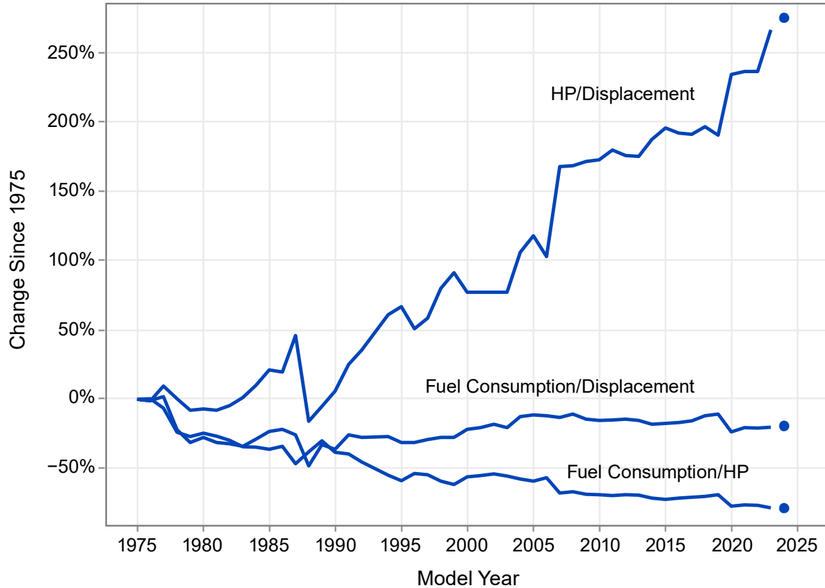
Figure 4.23. Percent Change for Specific Diesel Engine Metrics
