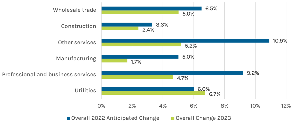
Figure 7. Electric Power Generation Actual Employment Change 2022-2023 vs. Anticipated Employment Change 2022
